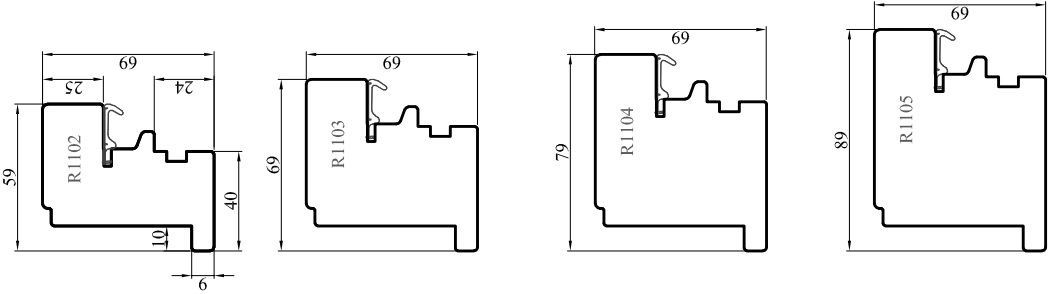
Dormant standard
