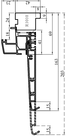
Appui aluminium
